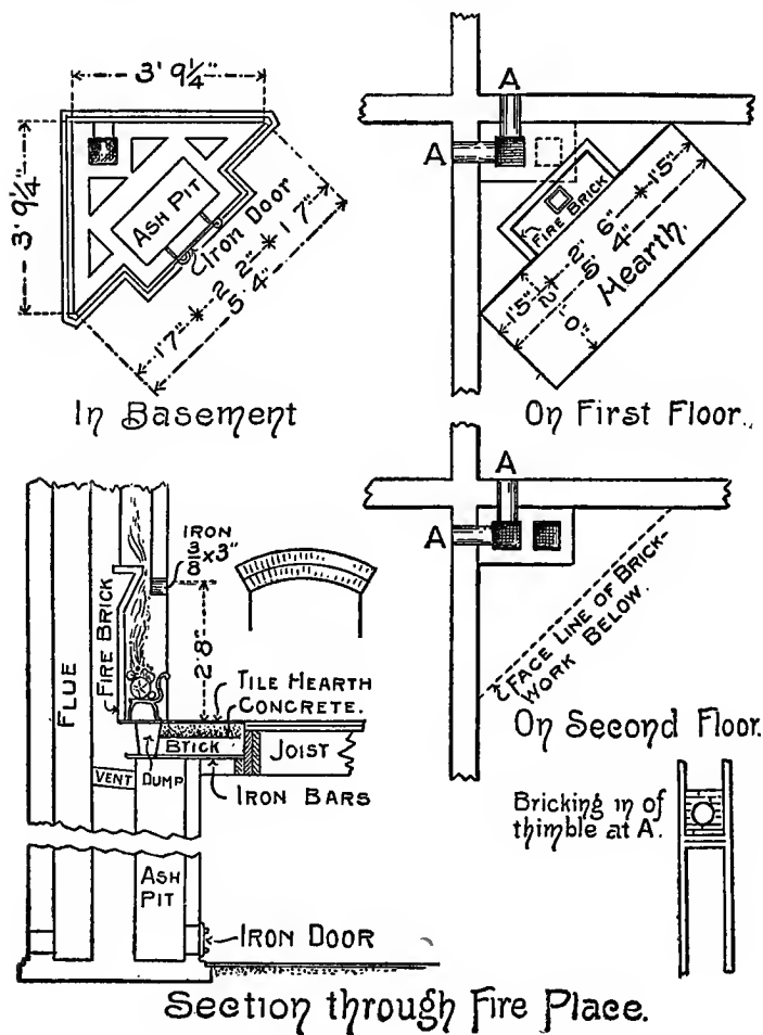
Fig. 46. Arrangement for Fireplace.
