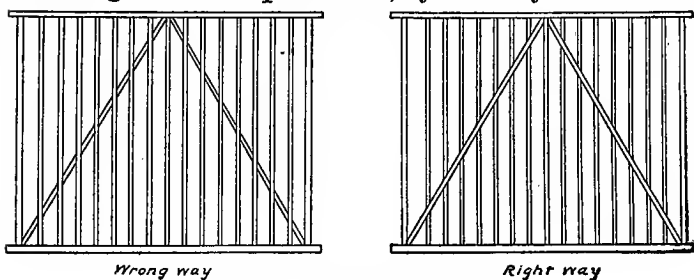
Fig. 17. Bracing a Partition.
