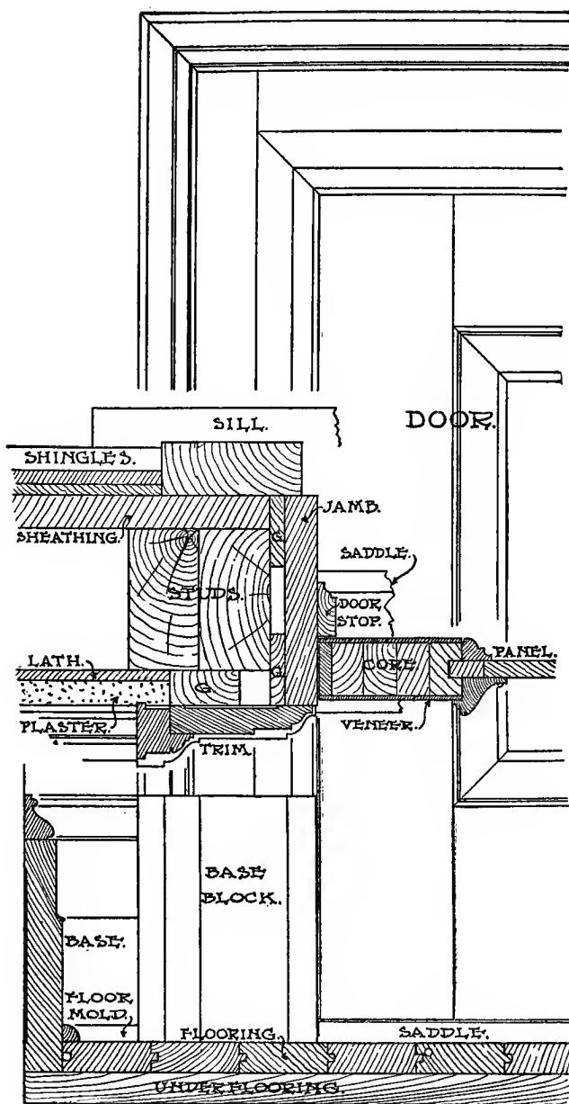
Fig. 37. Framing for Exterior Door.
