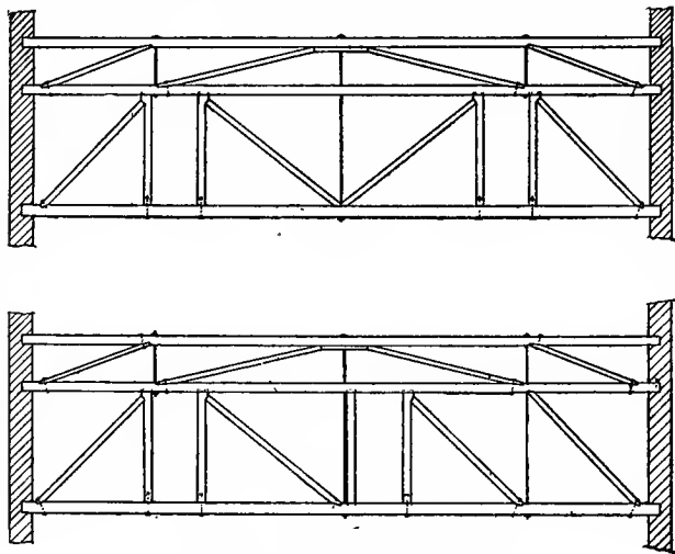
Fig. 182. Trussed Partitions.
