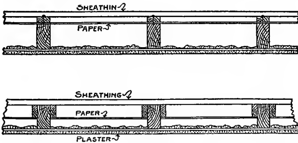
Fig. 15. Wall Sections, Showing Use of Paper Backing.
