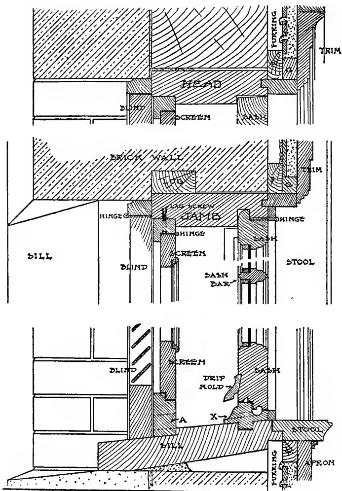
Fig. 100. Casement, Screen, and Blind in Brick Wall.
