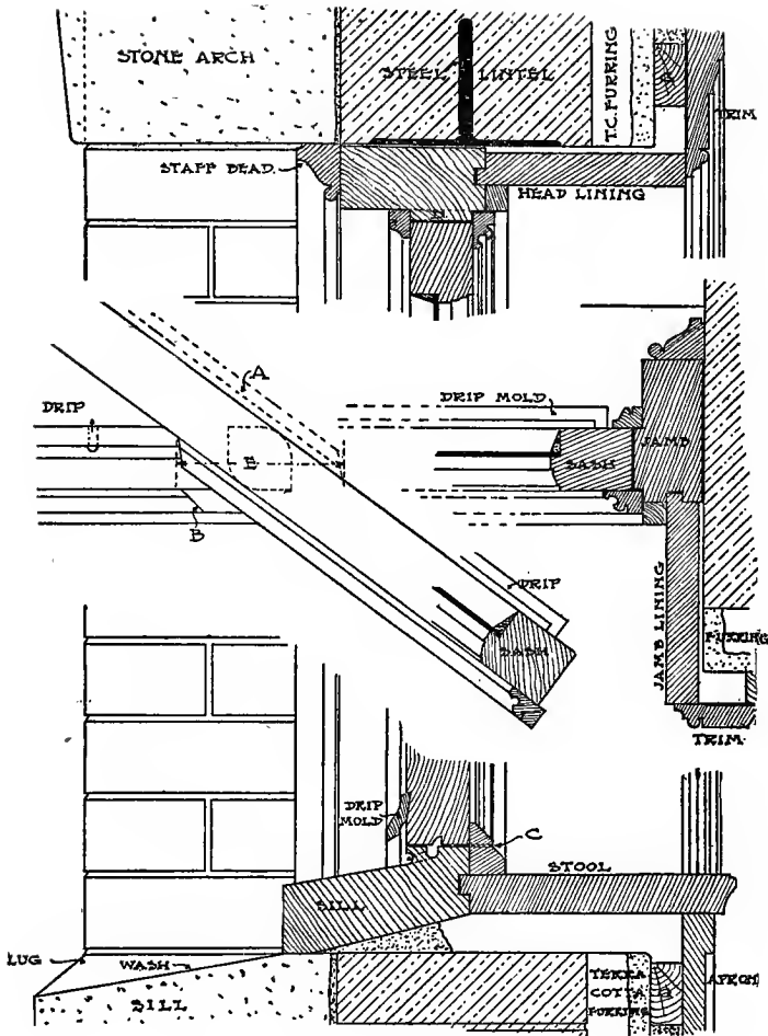
Fig. 105. Pivoted Casement Window.
