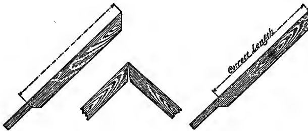
Fig. 58. Wrong and Right Methods of Figuring Rafter Lengths.
