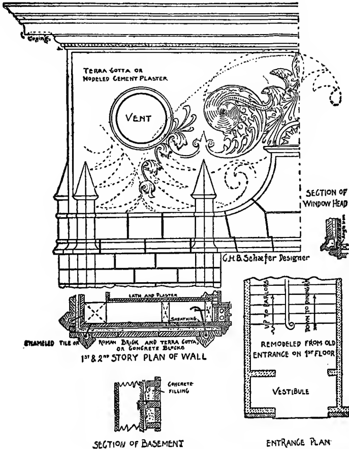
Fig. 109. Design and Construction for Tile Veneer Remodeling.
