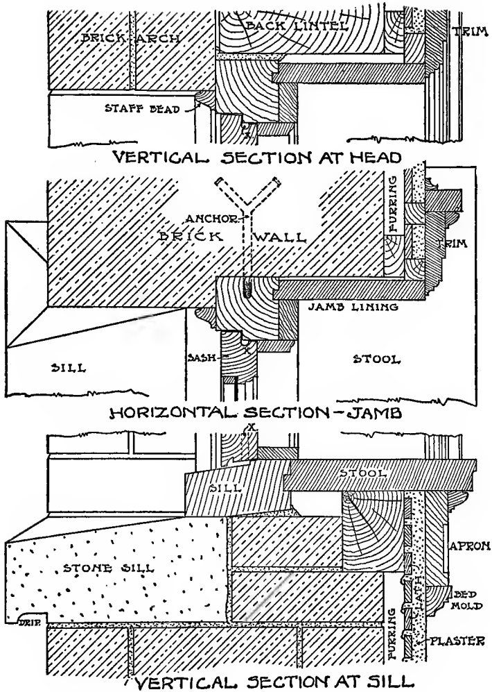
Fig. 97. Casement Window in 16-Inch Brick Wall.
