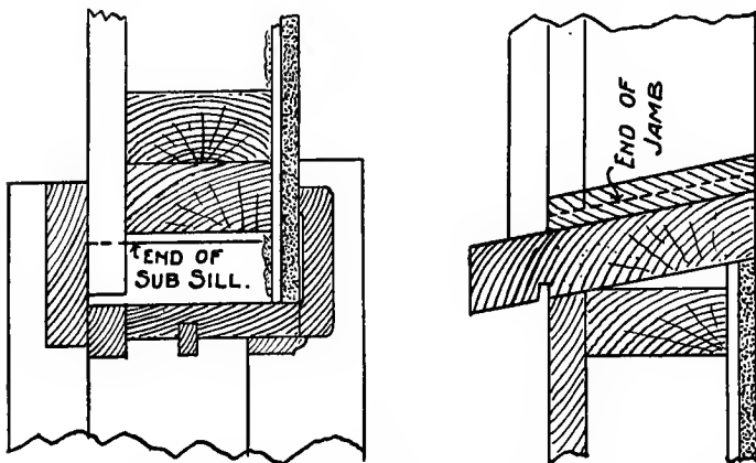
Fig. 22. Simple Window Construction.
