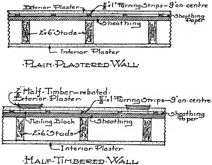
Fig. 91. Wall Sections—Cement Plaster Houses.
