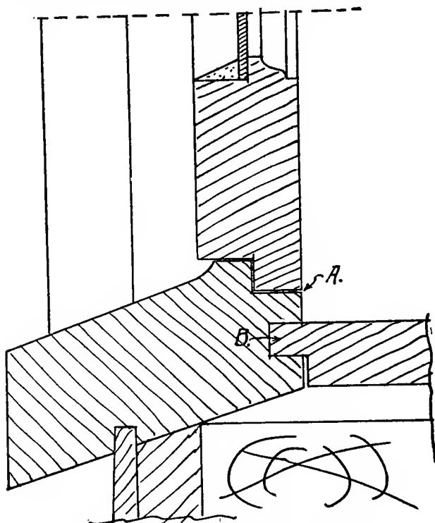
Fig. 23. Framing for Single-Sash Windows.
