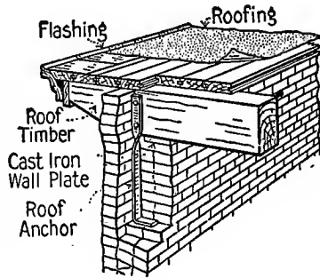
Fig. 155. Roof Timber Resting on Cast-Iron Wall-Plate, Showing Overhanging Open Wood Cornice and Wrought-Iron Anchor.
