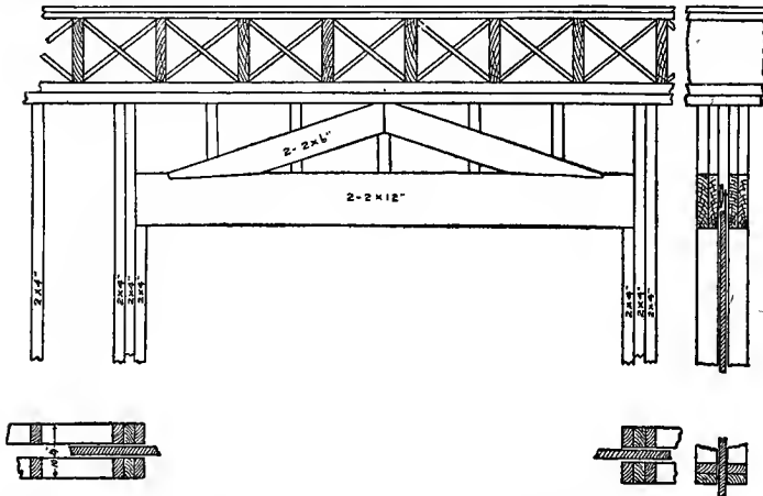
Fig. 16. Double Trussed Partition for Sliding Doors.
