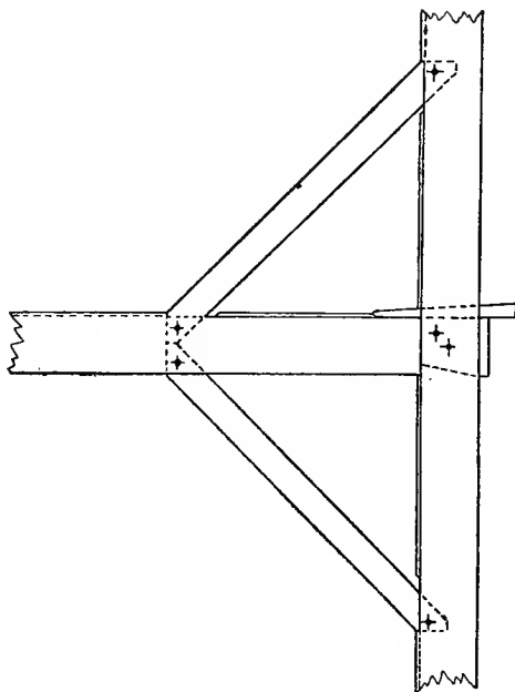
Fig. 125. Mortise Joint for Cross-Tie.
