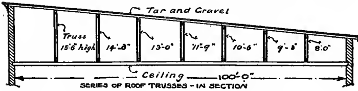
Fig. 177. How to Support a Flat Roof.
