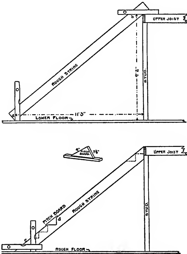
Fig. 86. Short Cut for Laying Out a Straight Stair.
