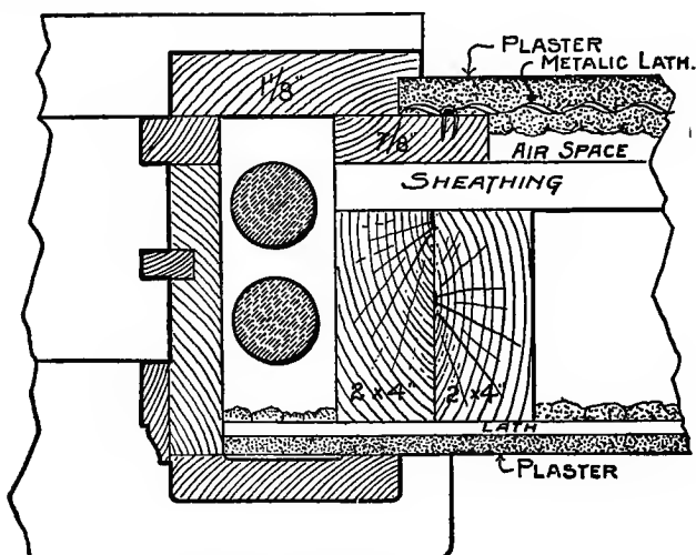
Fig. 92. Framing for Windows, Cement Plaster House.
