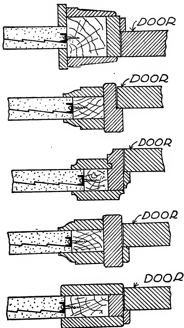
Fig. 117. Door Framing in Plaster Partitions.
