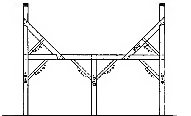
Fig. 123. Bracing to Prevent Outward Spreading.
