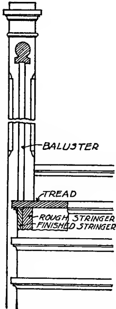
Fig. 83. Relation of Post, Rail, and String.
