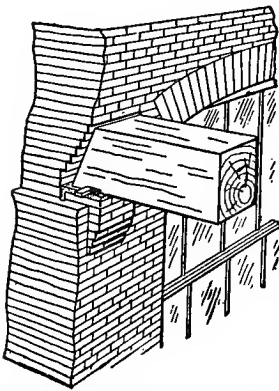
Fig. 153. Floor Timber Resting on Cast-Iron Wall-Plates, with Lugs for Anchoring Timber to Wall.
