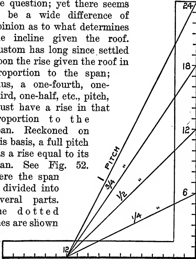
Fig. 53. Roof Pitches on the Steel Square.
