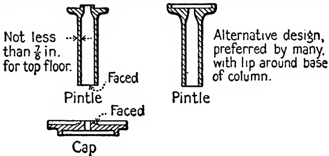
Fig. 157. Cap and Pintle Cast to Fit Columns.
