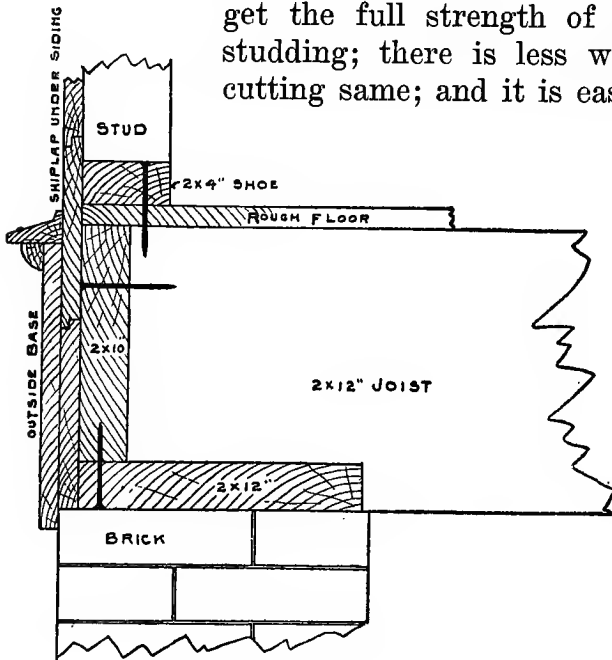
Fig. 10. Box Sill Construction.
