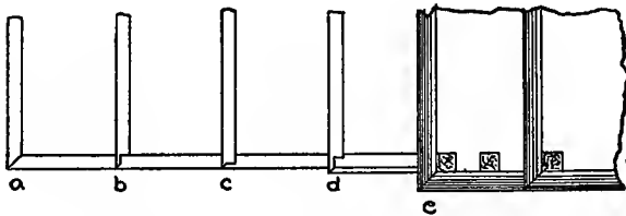
Fig. 78. Miter Joints for Open Stair Work.
