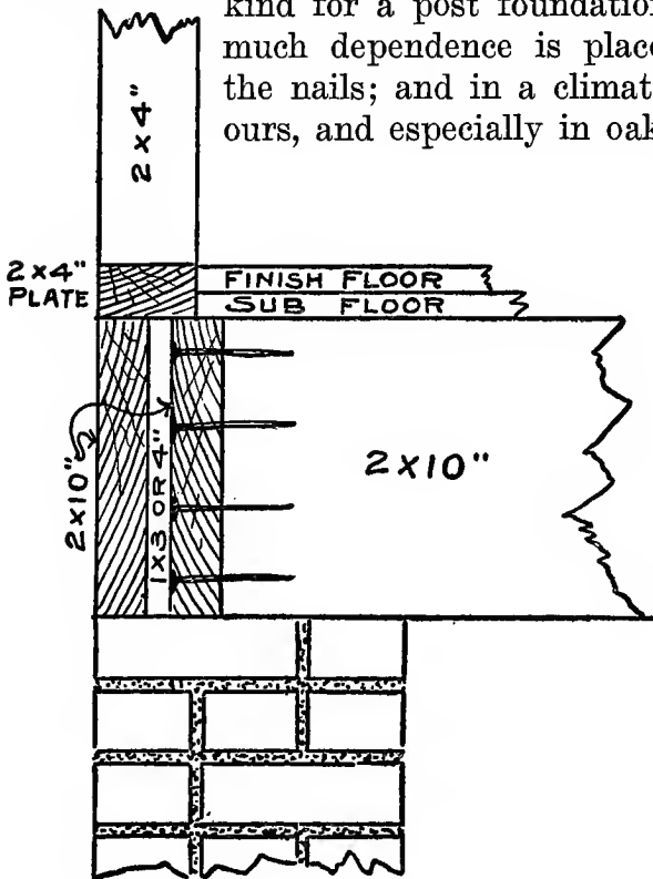
Fig. 9. A Built-Up Sill.
