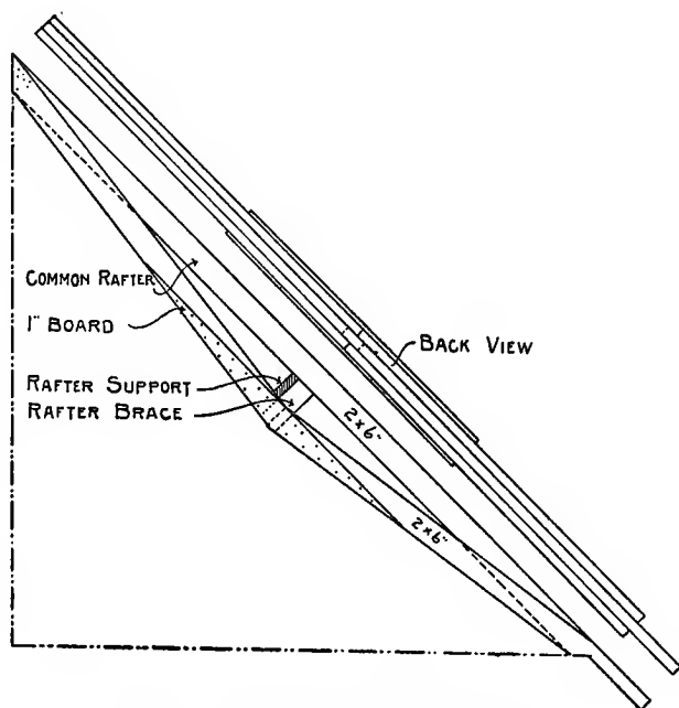
Fig. 135. Queen Rafter for Roof Support.
