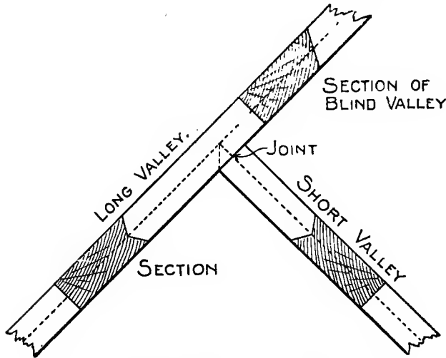
Fig. 60. Intersection of Valleys—Roof Dormers.
