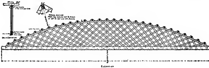
Fig. 176. Cheap Lattice Truss.
