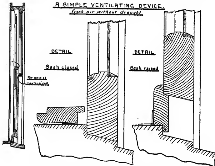
Fig. 32. Arrangement for Window Ventilating.
