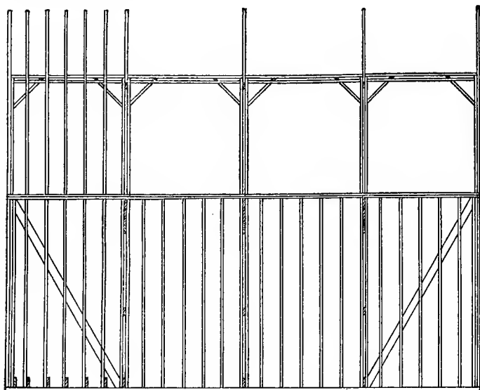
Fig. 133. Side Wall Plank Framing.
