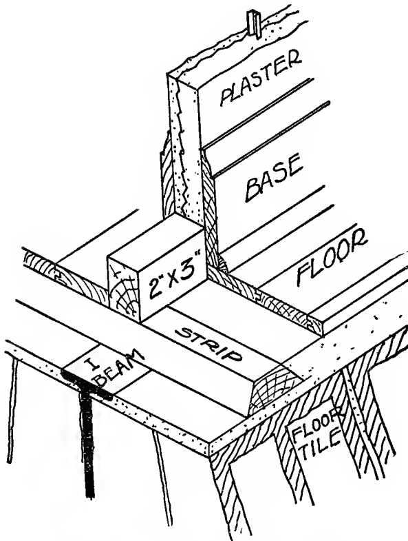
Fig. 118. Baseboard and Floor Construction.
