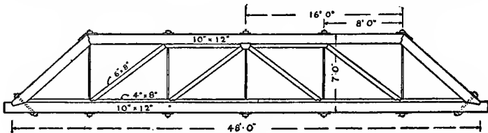
Fig. 181. Simple Wood Truss to be Cambered Two Inches.
