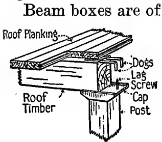
Fig. 154. Roof Timber Resting on Column Cap—Timbers Held Together by 1-Inch Wrought-Iron Dogs.
