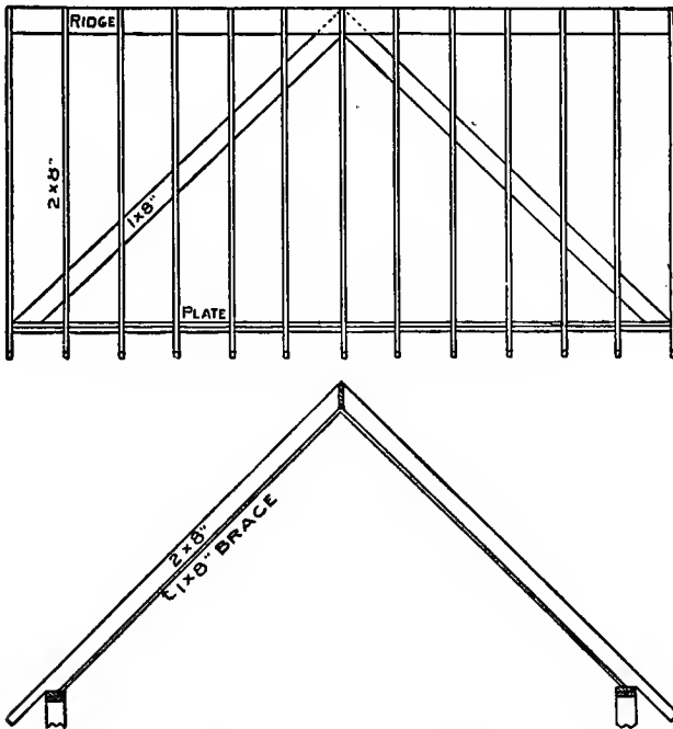
Fig. 67. Good Brace for Ridge.
