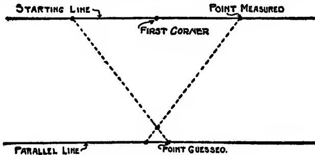
Fig. 2. Method of Squaring Work.
