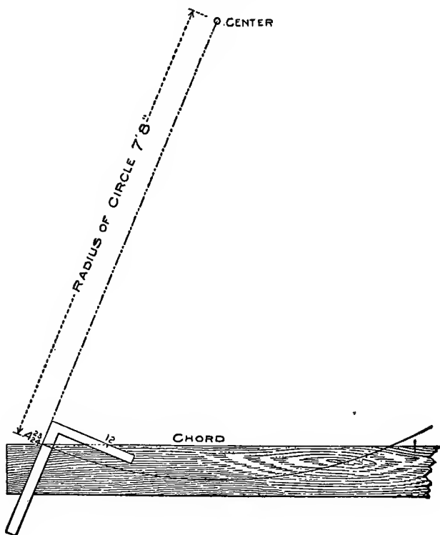
Fig. 42. How to Lay Out Circular Porch Work.
