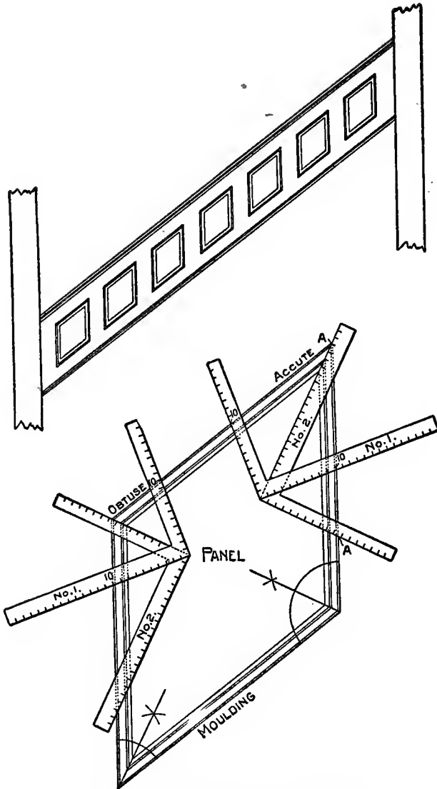
Fig. 87. Paneled Finish for Stairs.
