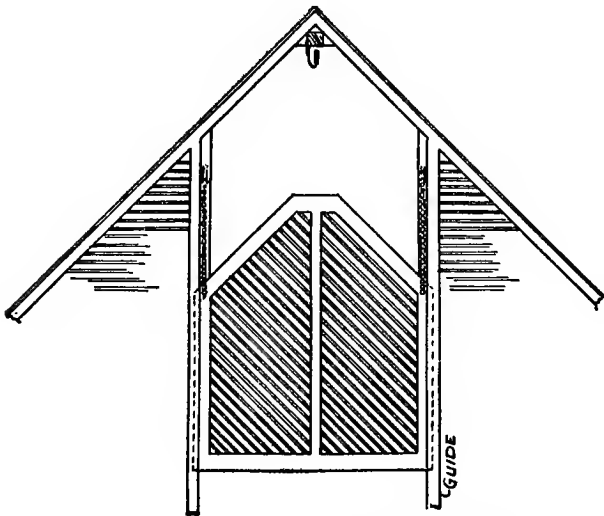
Fig. 141. Hay Door Hung with Weights.
