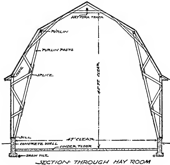
Fig. 138. Self-Supporting Roof Construction.
