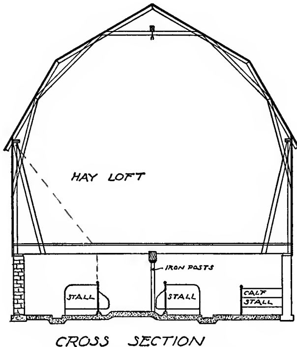
Fig. 137. Arrangement of Dairy Barn.
