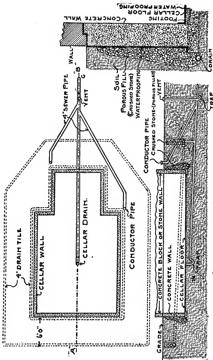
Fig. 5. Waterproofed Cellar with Drainage Piping.
