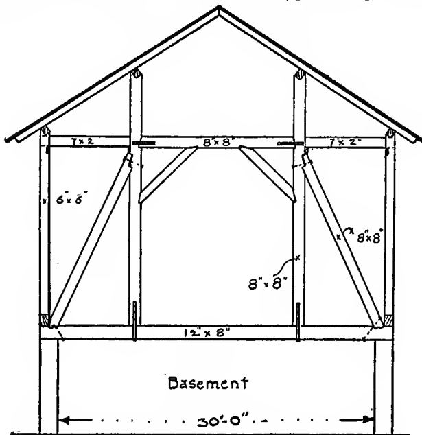
Fig. 121. Truss for Barn without Basement Posts.
