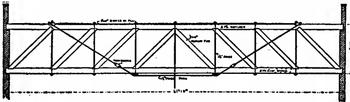
Fig. 180. Strengthening a Truss with Rods.
