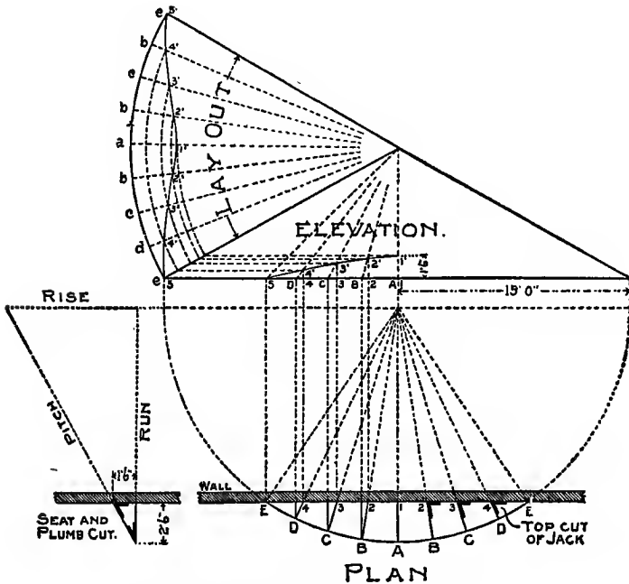
Fig. 63. How to Roof a Circular Bay.
