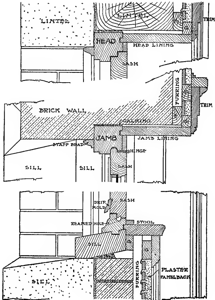
Fig. 99. Storm-Proof Inward-Opening Casement.
