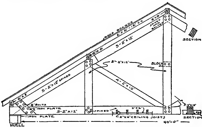
Fig. 174. Cheap Plank-Framed Truss.
