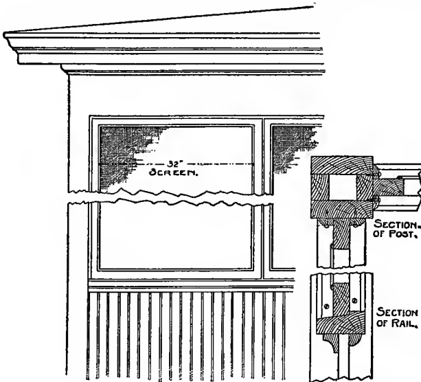
Fig. 40. Construction and Design of a Screened Porch.
