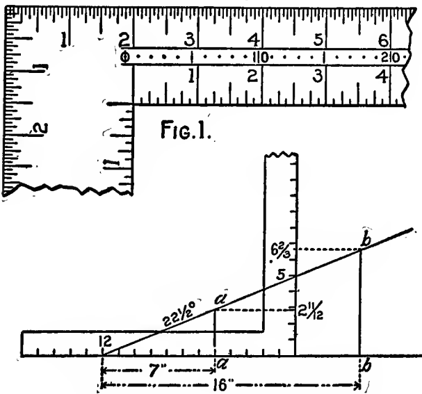
Fig. 65. Octagon Scale and Another Method.
