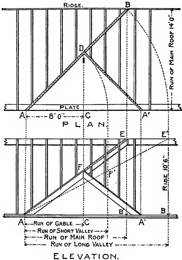
Fig. 59. Framing for Roof Dormers.
