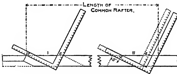
Fig. 55. Getting the Length of Rafters.
