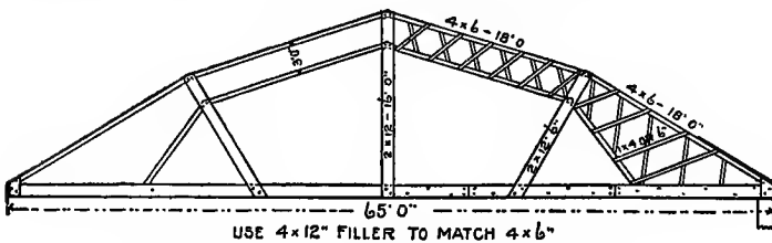
Fig. 173. Cheap Roof Truss for Broad Span.
