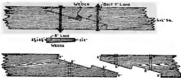
Fig. 130. Good Splice for Heavy Timbers.
