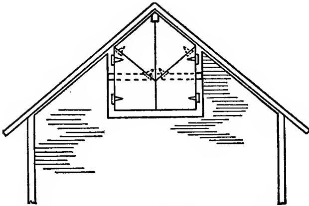
Fig. 143. Double Doors to Swing and Fold Down.
