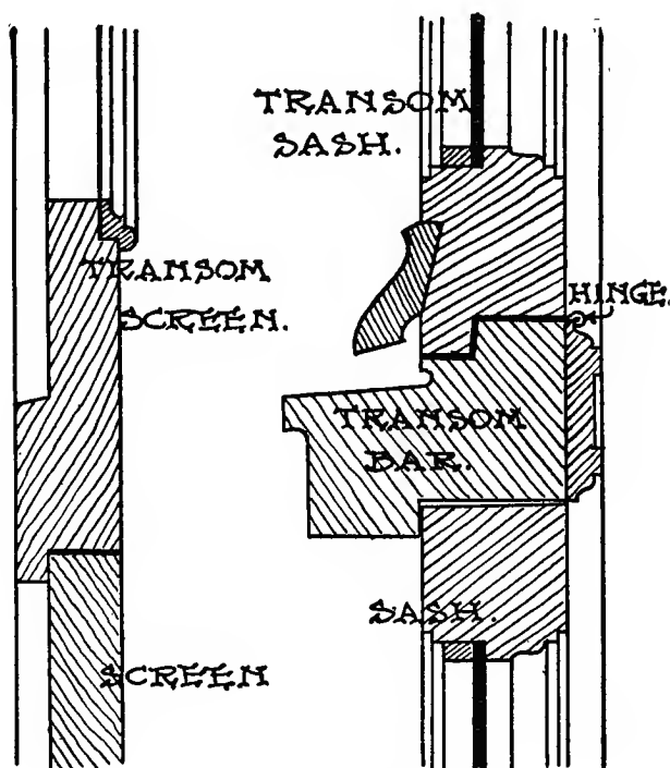
Fig. 101. Section at Transom.
