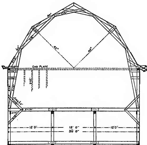
Fig. 136. Plank-Framed Truss for Gambrel Roof.
