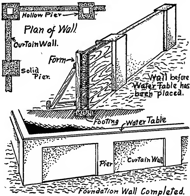
Fig. 4. An Economical Concrete Foundation.
