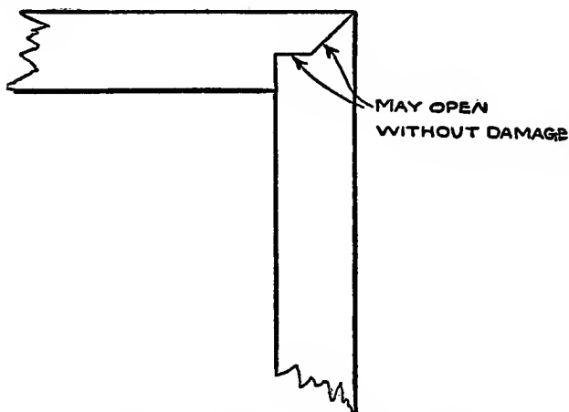
Fig. 45. Miter Joint for Solid Porch Plate.
