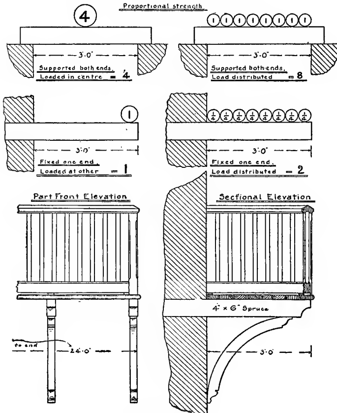
Fig. 164. Strength of a Projecting Veranda.
