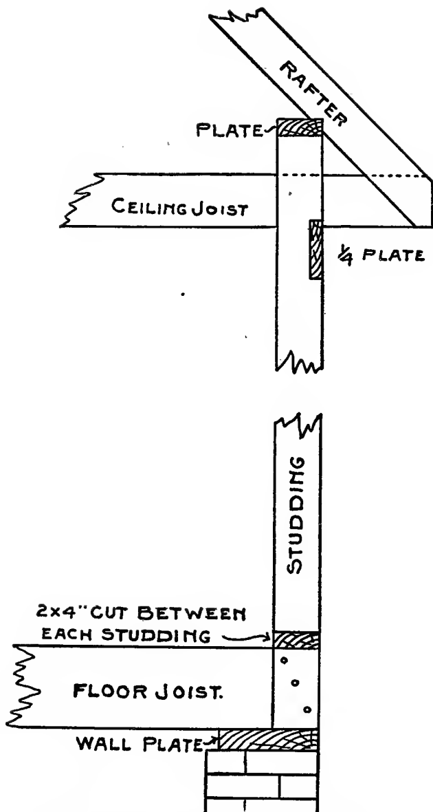
Fig. 13. Wall Construction, Sill to Plate, in Small House.
