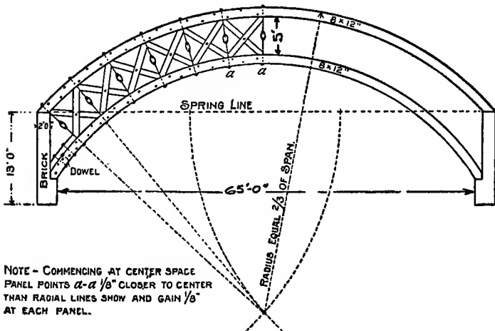
Fig. 172. Strong, Curved Roof Truss.
