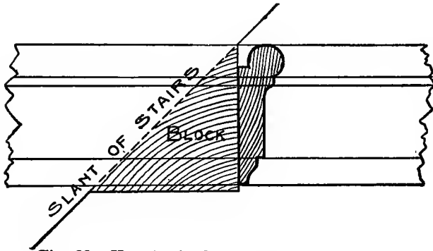
Fig. 88. How to Apply Moulding under Stairs.
