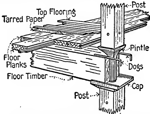
Fig. 156. Cast-Iron Cap and Pintle for Columns and Dogs for Holding Floor Timbers Together.
