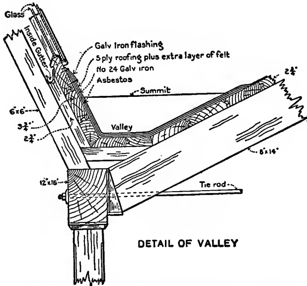
Fig. 160. Saw-Tooth Roof Framing—Detail of Valleys.
