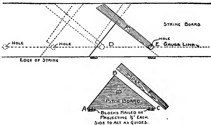
Fig. 75. Method of Laying Out Stair Strings.
