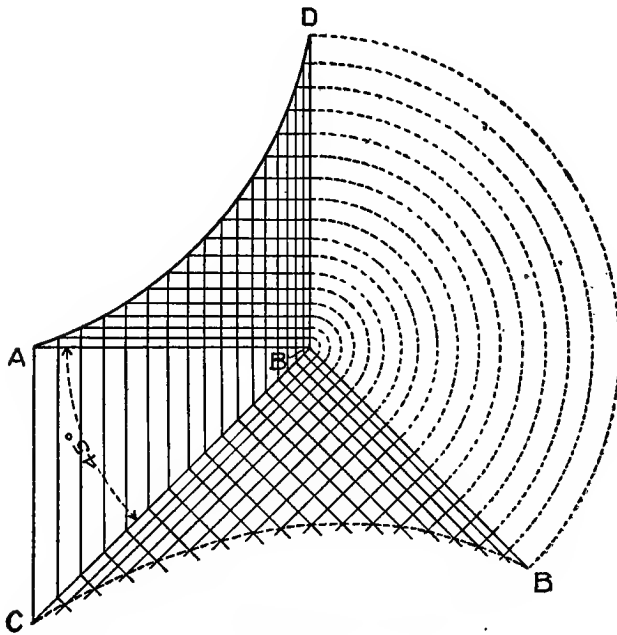
Fig. 64. Developing Curved Hip Rafter.
