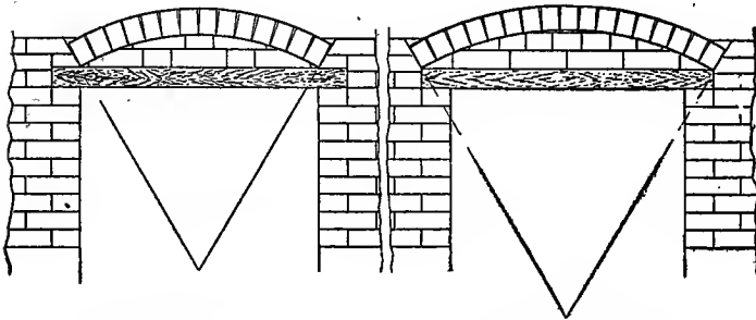
RELIEVING ARCH WRONG METHOD
