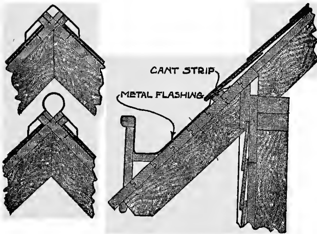
Fig. 119. Proper Construction at Ridge and Eaves for Slate.
