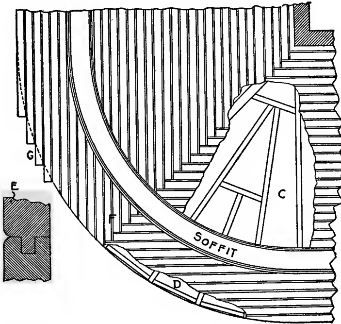
Fig. 44. Ceiling and Roof Framing—Circular Porch.
