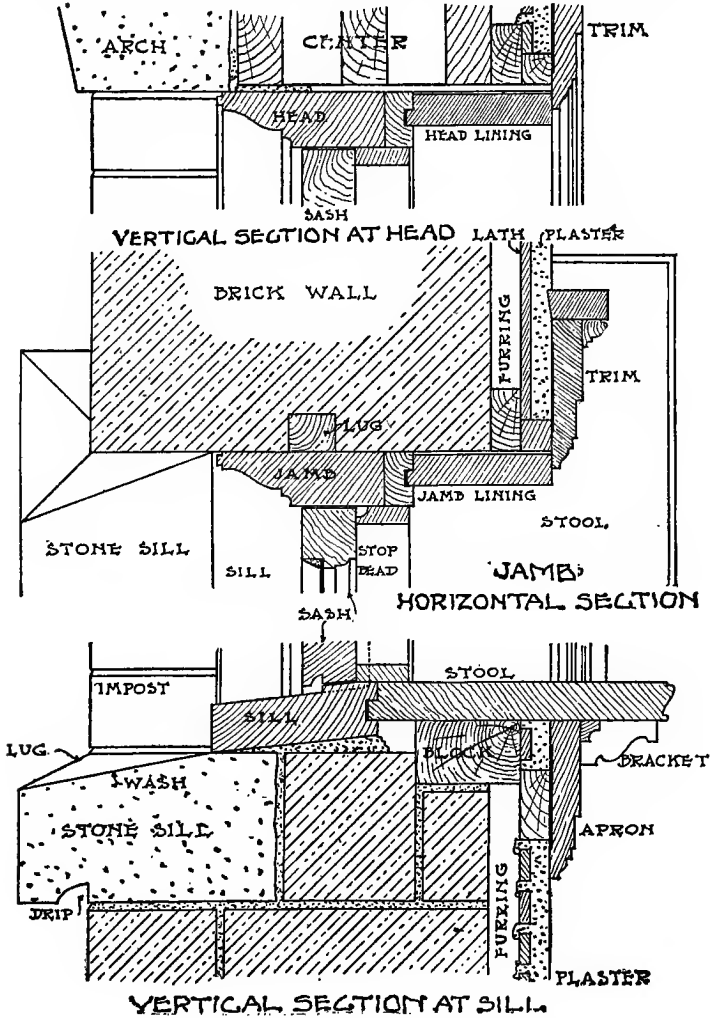
Fig. 96. Casement Window in 13-Inch Brick Wall.
