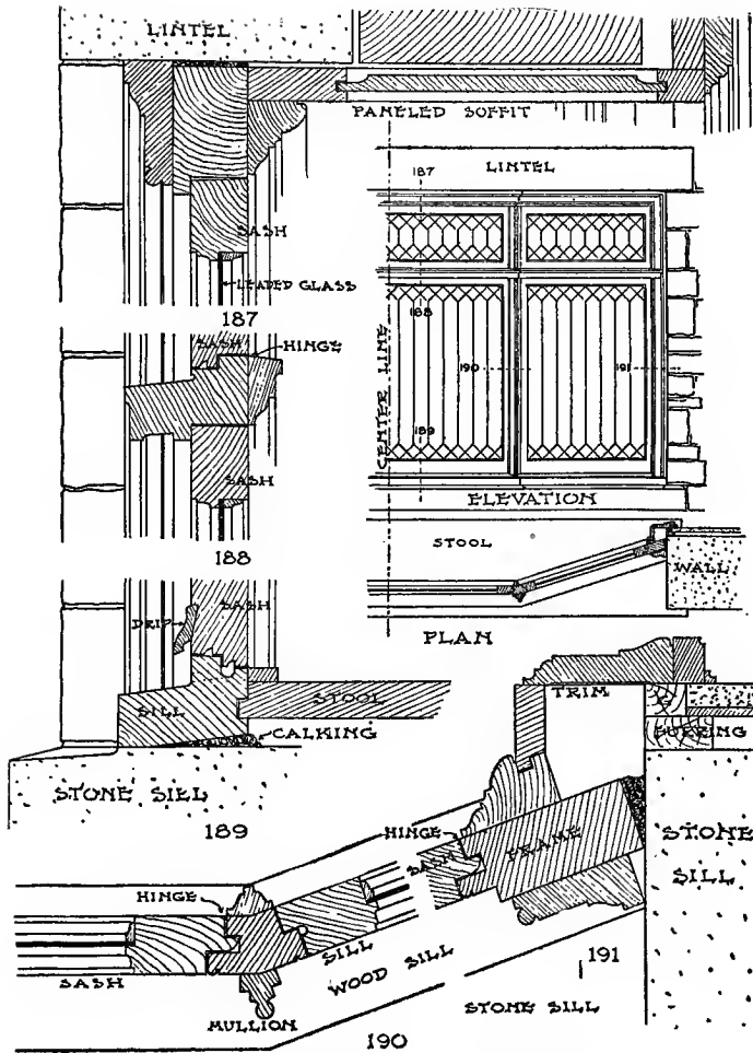
Fig 103. Inward-Opening Casement Bay.
