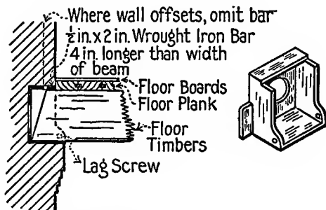
Fig. 152. Cast-Iron Wall Box for Floor Timbers, with Lugs for Anchoring to Walls.
