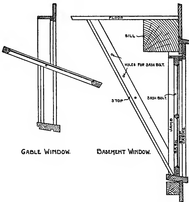
Figs. 147 and 148. Barn Gable and Basement Windows.
