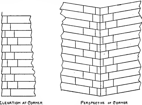
Fig. 48. Shingling a Corner.
