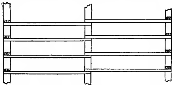
Fig. 12. Proper Arrangement of Joist and Sills.
