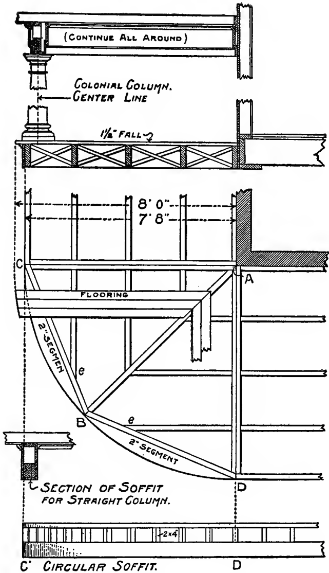
Fig. 41. Framing for Circular Porch.
