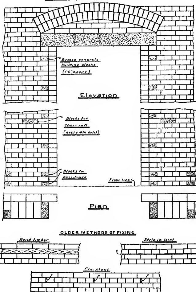
Fig. 114. Details of Fireproof Brick Construction.
