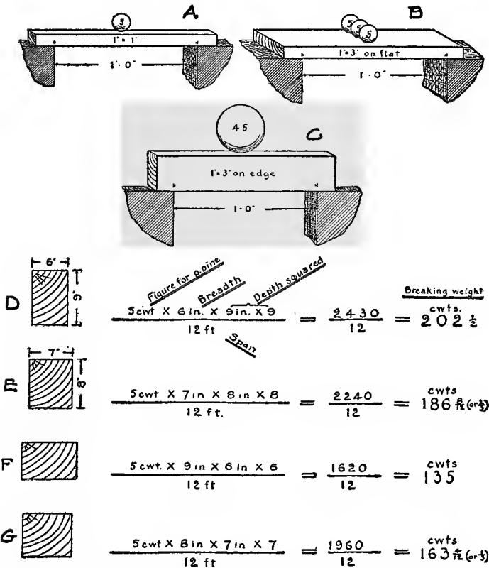
Fig. 161. Ultimate Strength of Beams Supported at Both Ends with Load Concentrated at the Middle.
