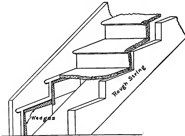
Fig. 73. Housed-String Stair Construction.
