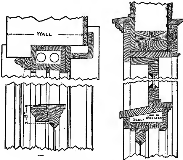
Fig. 29. Framing for Transom Windows.
