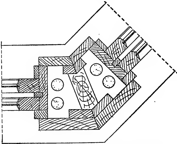
Fig. 31. Construction at Corner, Octagon Bay.
