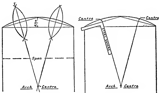
Fig. 112. To Find the Arch Centers.
