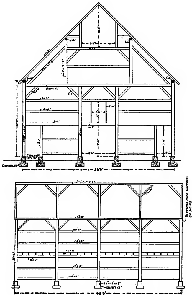
Fig. 128. End and Side Wall Framing for Hay Barn.
