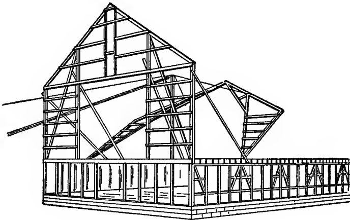
Fig. 134. How the Bents are Raised.
