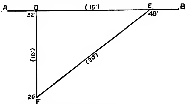
Fig. 1. Squaring Work by the 6, 8, and 10 Rule.
