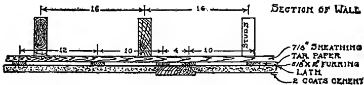
Fig. 90. Wall Section, Plastered House, Half-Timber Effect.
