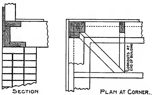
Fig. 7. Box Sill Construction.
