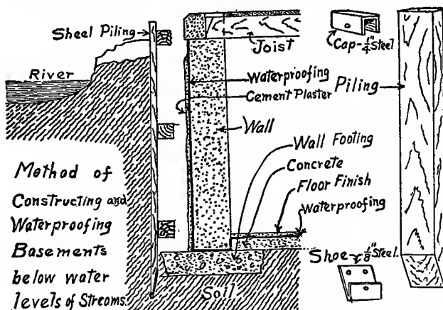
Fig. 6. Waterproofing Cellars below Water Level.
