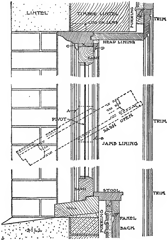
Fig. 104. Pivoted Casement Window.
