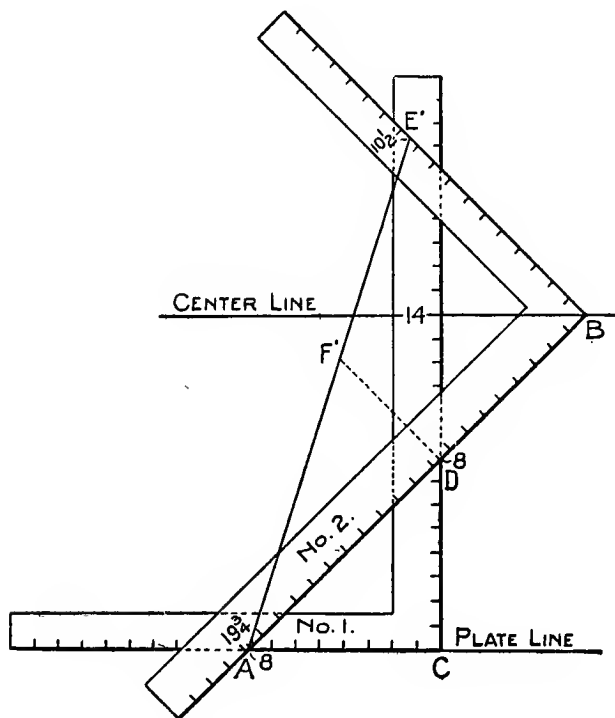
Fig. 62. Steel Square in Roof Dormer Framing.
