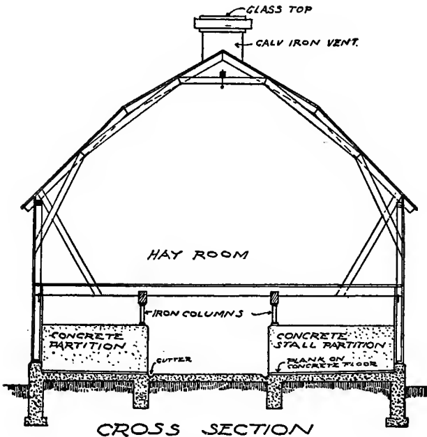
Fig. 139. Concrete Stable Floor and Partitions.
