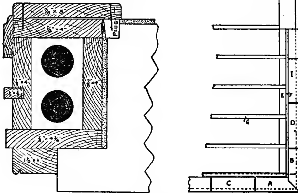
Fig. 107. Wood Framing with Concrete Blocks.
