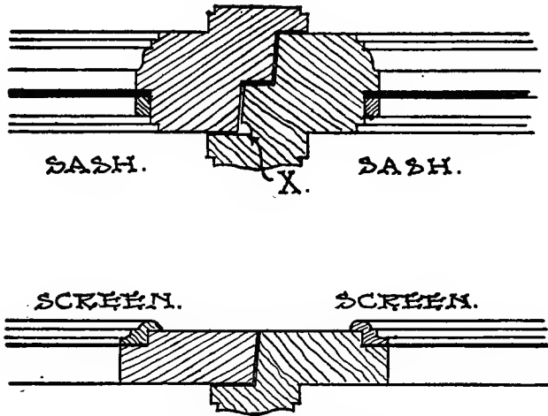
Fig. 102. Section at Meeting Rails.
