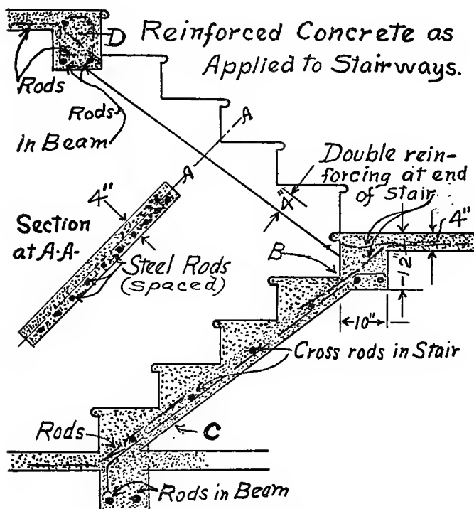
Fig. 116. Details, Concrete Fireproof Stairs.
