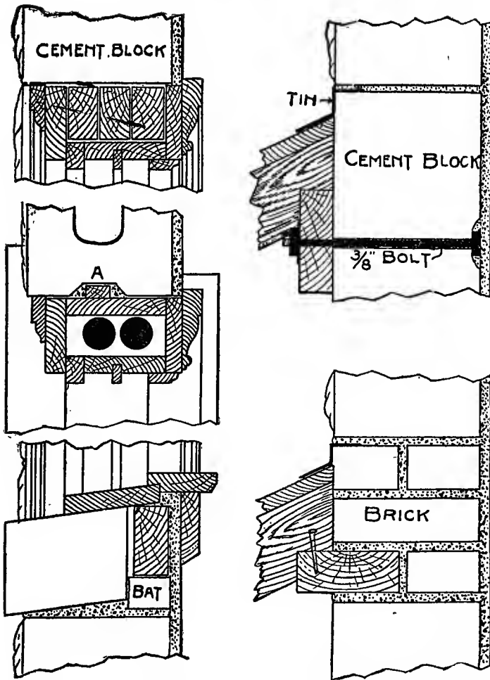
Fig. 106. How to Arrange Window-Frames and Attach Porch Roof.
