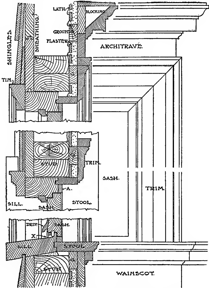
Fig. 26. Framing for Inward-Opening Casements.
