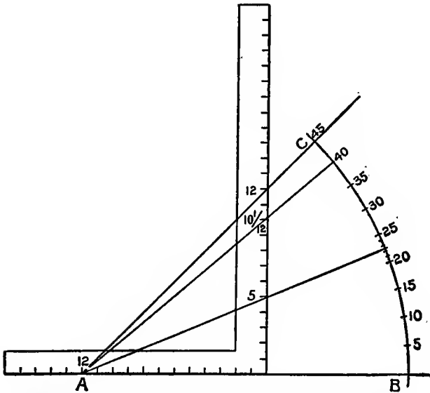
Fig. 66. To Lay Out an Angle with the Steel Square.
