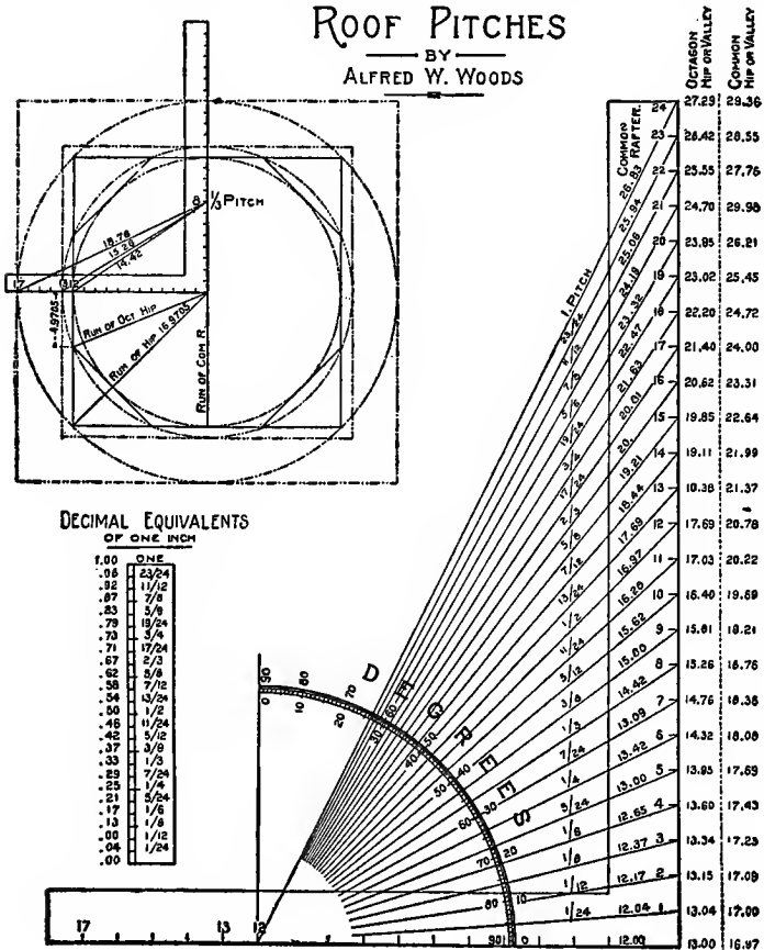
Fig. 51. Roof Pitches and Degrees on the Steel Square.
