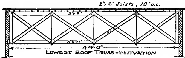
Fig. 178. Truss for Flat Roof.
