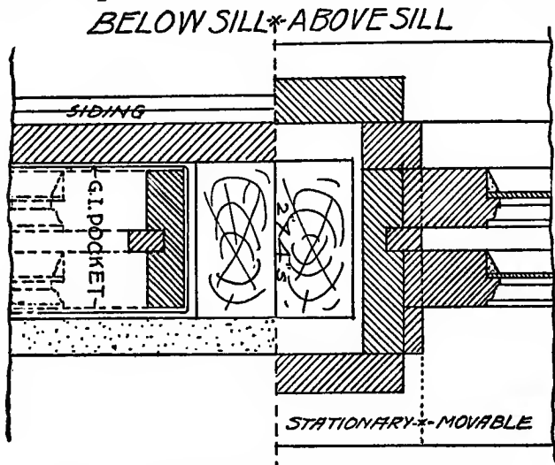
Fig. 34. Detail Window Jambs for "Open-Air" Room.
