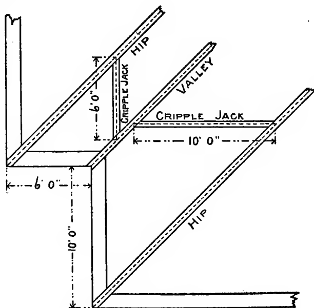
Fig. 56. Cripple Jack Rafters in Place.
