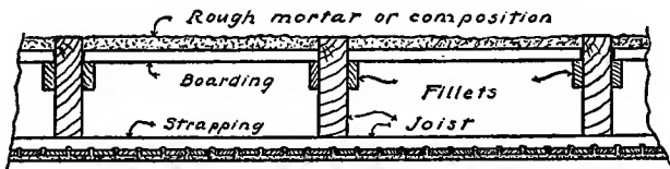
Fig. 68. Ceiling Construction to Prevent Heat Losses.
