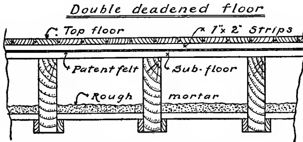
Fig. 179. Method of Deadening Floor for Rink.
