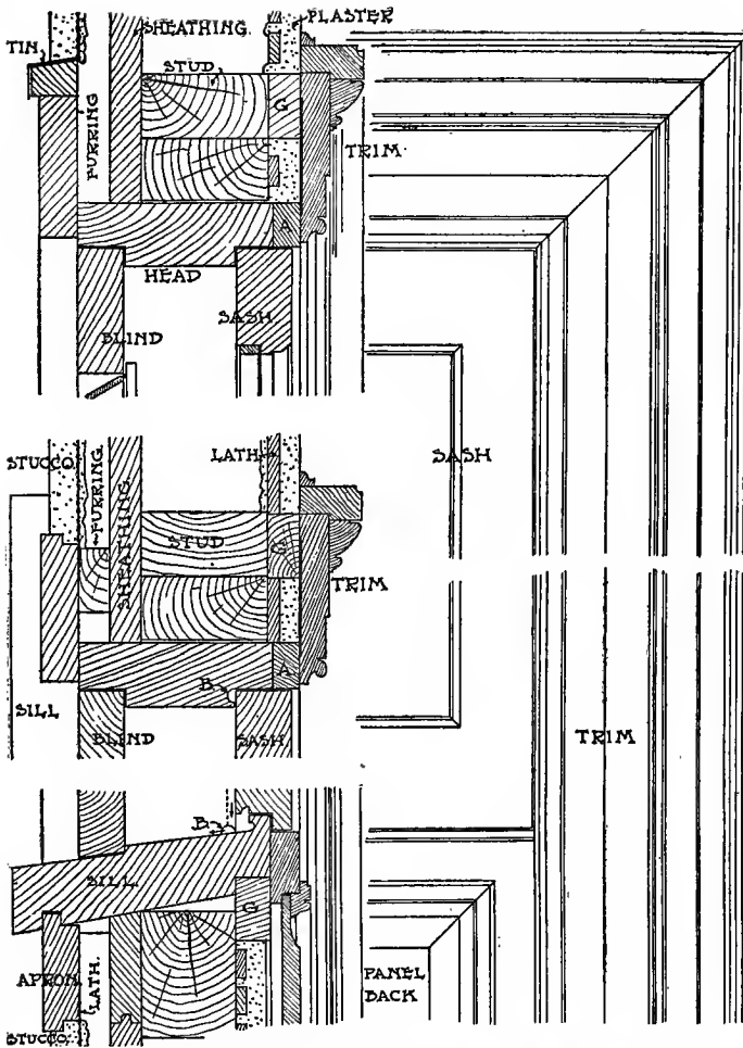
Fig. 93. Casement Window in Cement Plaster House.
