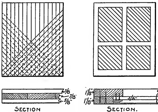
Fig. 140. How to Make a Heavy Barn Door.
