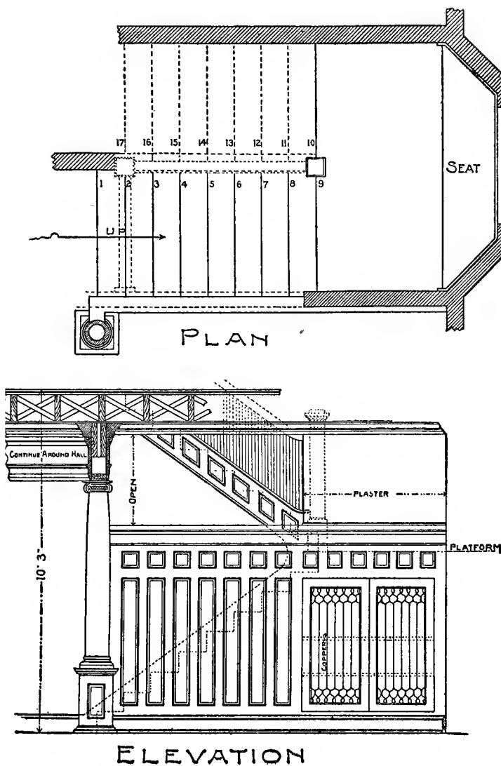
Fig. 81. Desirable Stair Arrangement for Residences.
