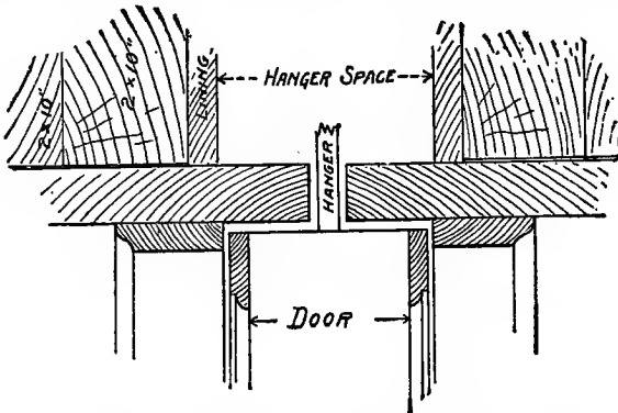
Fig. 39. Sliding Doors—Construction at Head.
