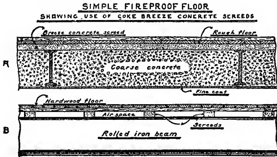
Fig. 115. Details of Fireproof Construction.
