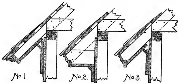
Fig. 19. Cornice Construction.
