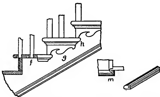
Fig. 79. Construction and Finish of Open Stairs.
