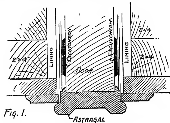
Fig. 38. Sliding Doors—Construction at Jamb.
