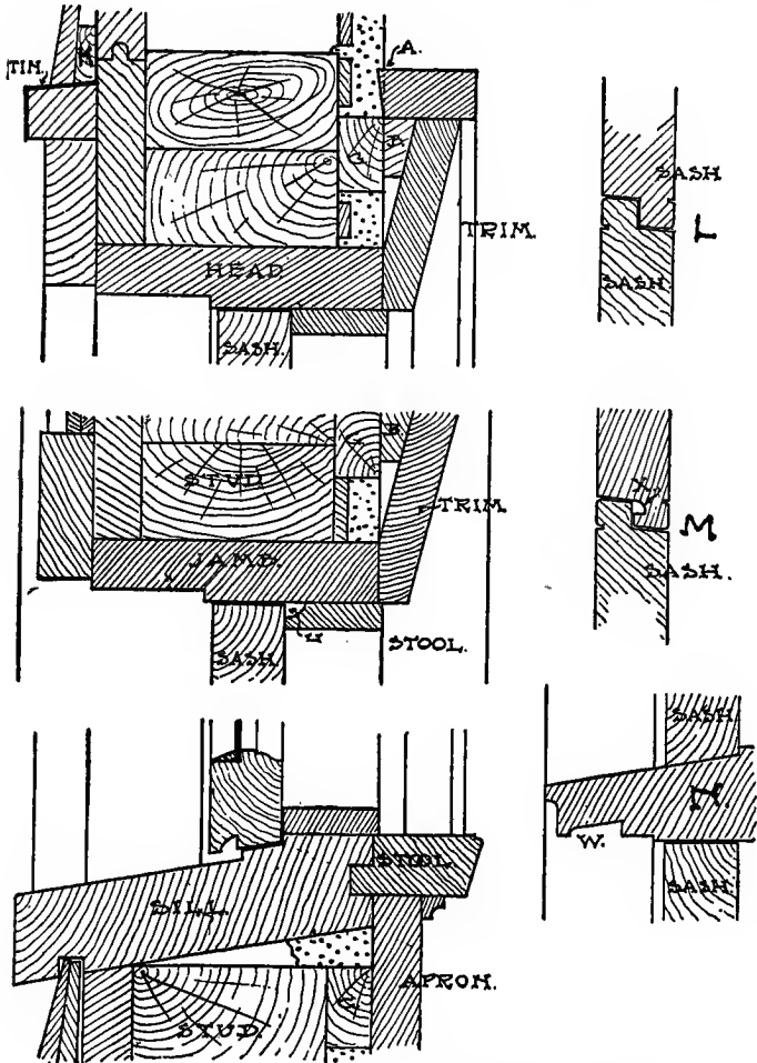
Fig. 24. Framing for Outward-Opening Casements.
