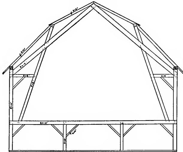
Fig. 129. Center Bent of Gambrel Roof Hay Barn.
