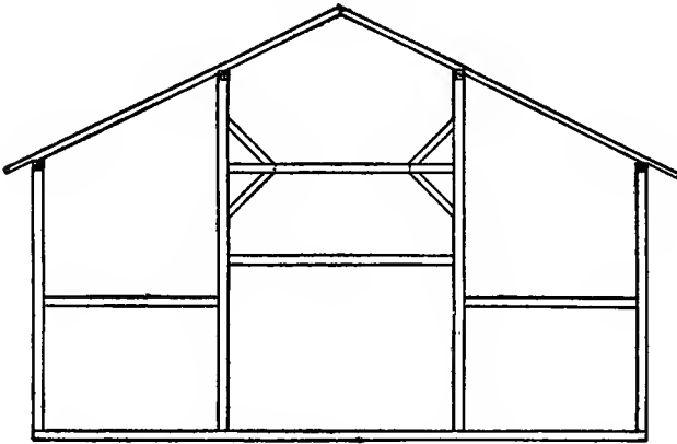
Fig. 124. Center Bent, Showing Purlin Post Bracing.
