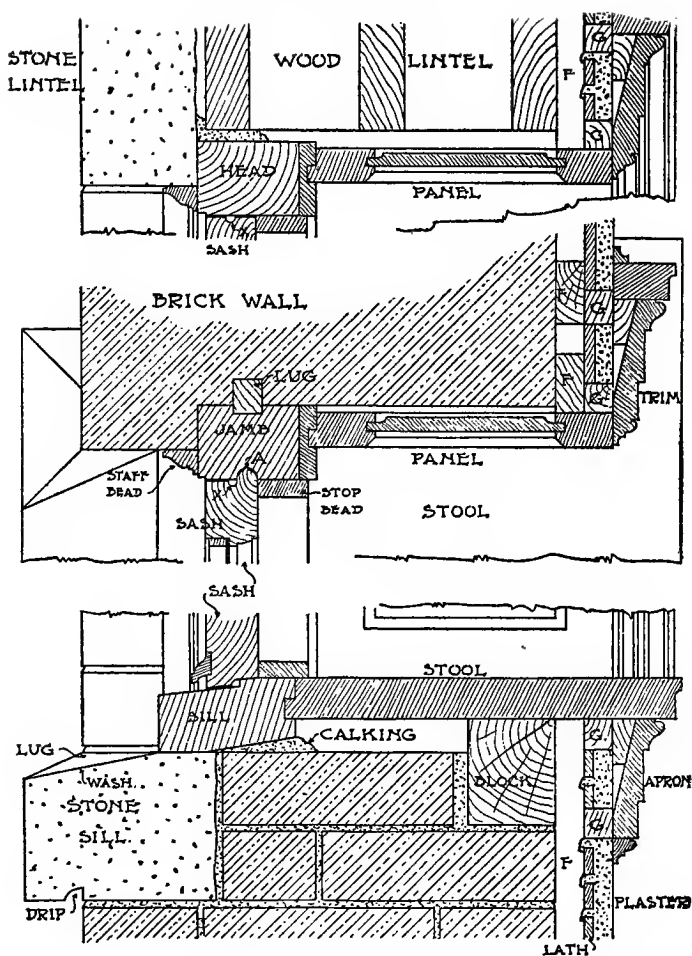
Fig. 98. Outward-Opening Casement in Brick Wall.
