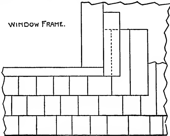
Fig. 50. Shingling Below a Window.
