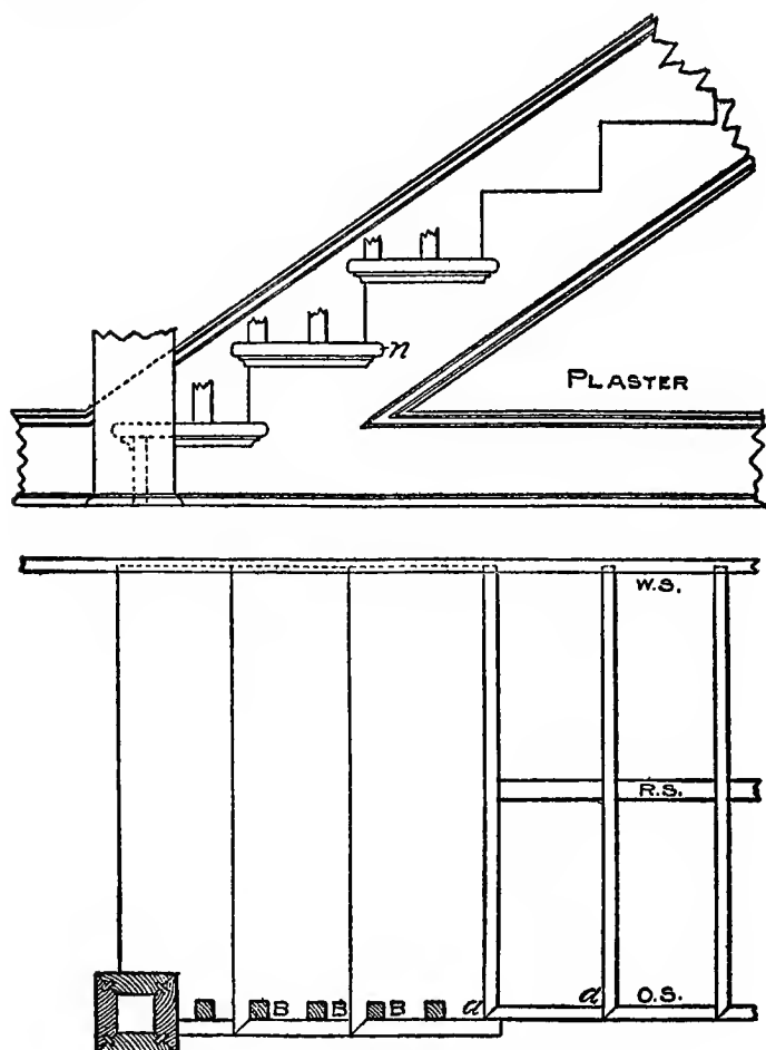
Fig. 77. Plan and Elevation of Open-String Stair.
