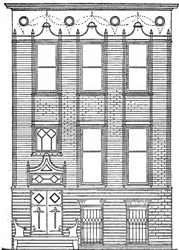
Fig. 108. Design for Remodeling and Veneering Old-Style Frame Fronts.
