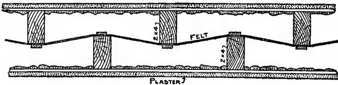
Fig. 14. An Inexpensive Sound-Proof Wall.
