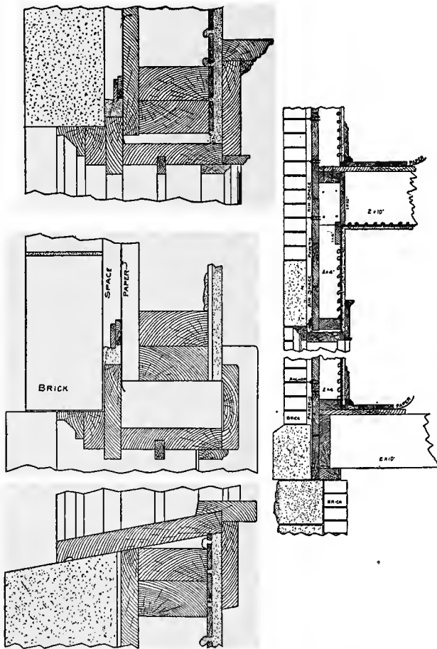
Fig. 95. Wall Section Showing Air Spaces and Framing.
