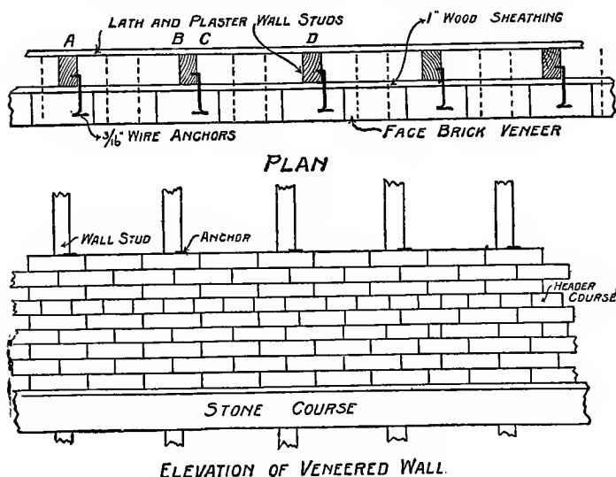
Fig. 94. Brick Veneer Wall Construction, Showing Bonding.
