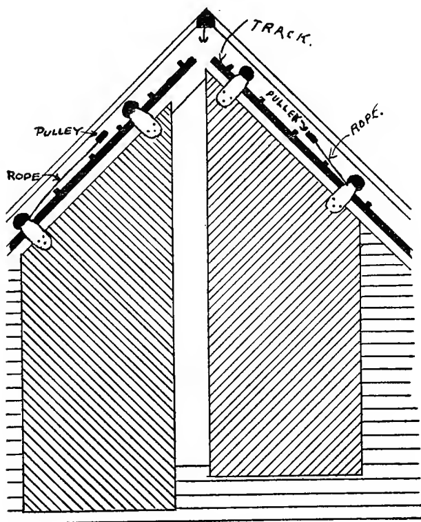
Fig. 144. Weighted Doors on Inclined Tracks.
