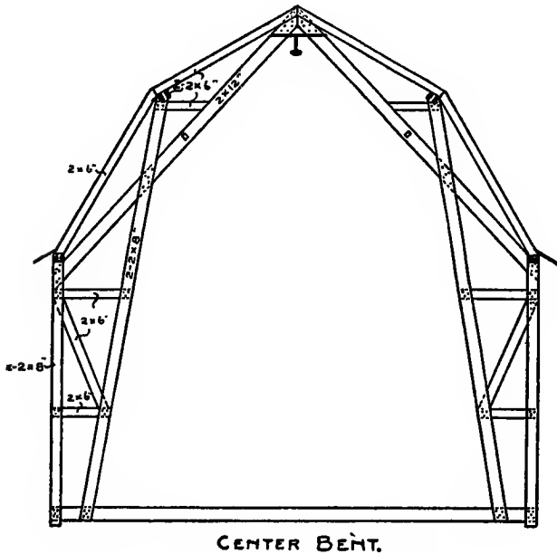
Fig. 132. Wind Bracing for Plank-Frame Barn.
