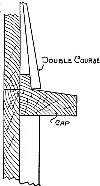
Fig. 49. Shingling Over a Window.
