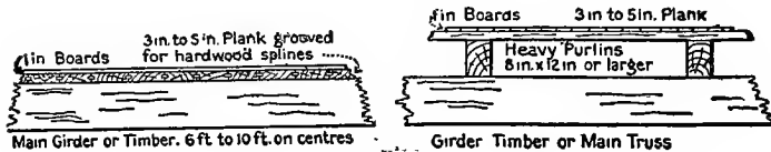
Fig. 151. Good Types of Floor Construction.
