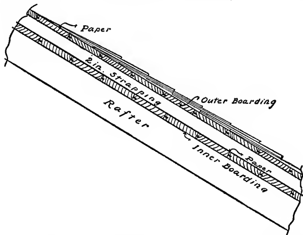
Fig. 69. Roof Construction to Prevent Heat Losses.
