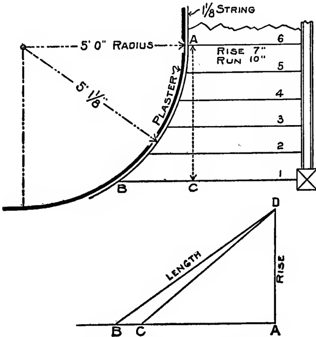
Fig. 84. Stair against a Circular Wall.
