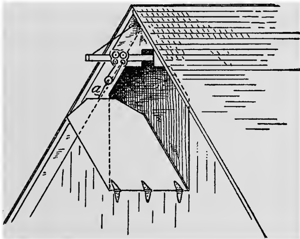
Fig. 145. Hay-Mow Door to Fold Down.
