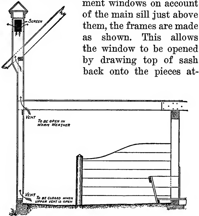
Fig. 146. How to Ventilate a Stable.
