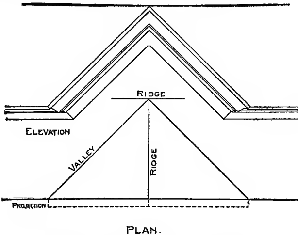
Fig. 20. Gable Flush with Side of House.
