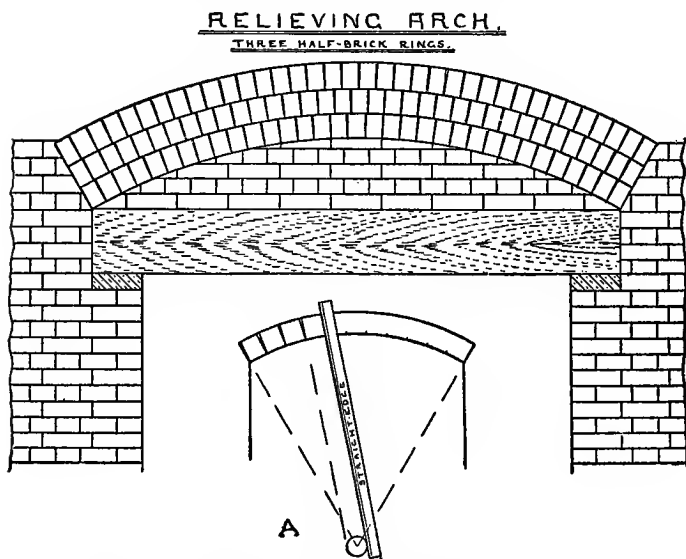
Fig. 111. Segmental Arch, and How to Lay It Out.
