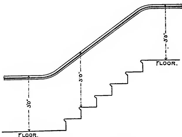
Fig. 89. Height of Wainscoting.
