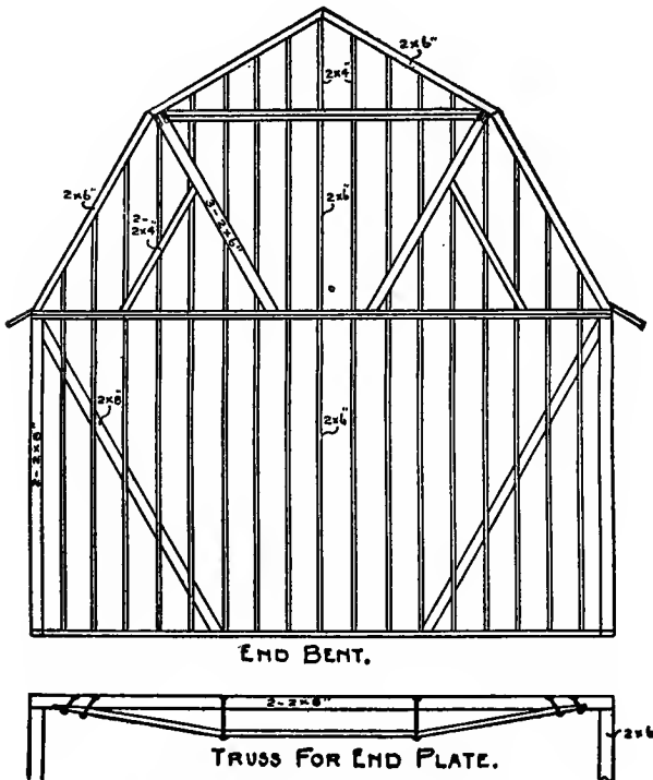
Fig. 131. Plank-Frame Construction.
