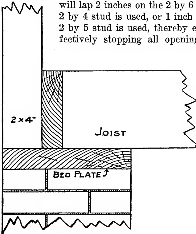
Fig. 8. Box Sill Construction.
