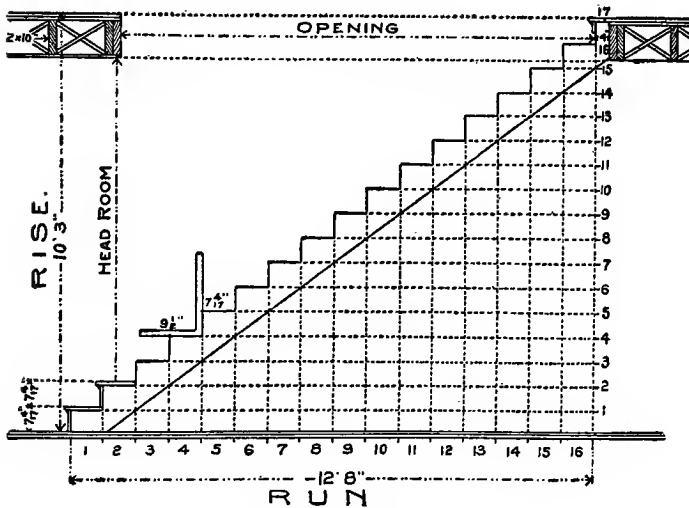
Fig. 71. Layout of Simple Stairs.
