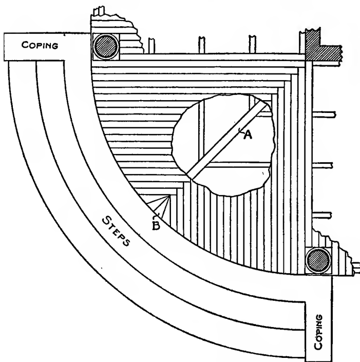
Fig. 43. Floor Construction—Circular Porch.
