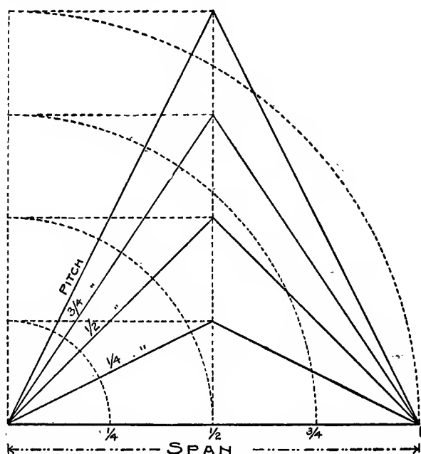
Fig. 52. Roof Pitches.
