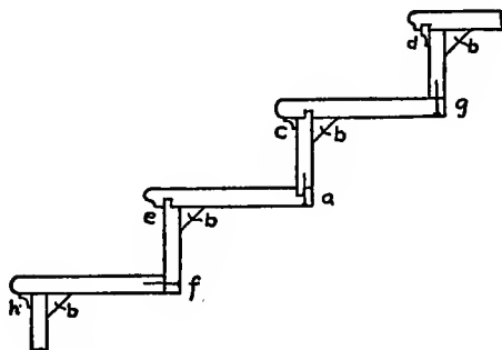
Fig. 76. Methods of Joining Risers and Treads.
