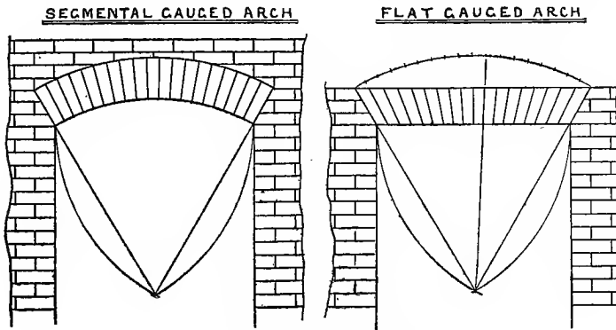
Fig. 113. Brick Arches.
