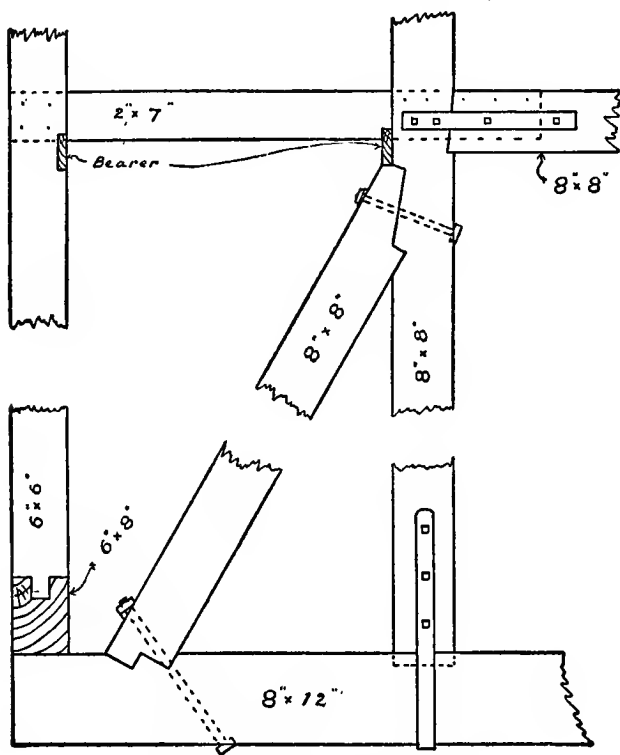
Fig. 122. Details of Heavy Framing.
