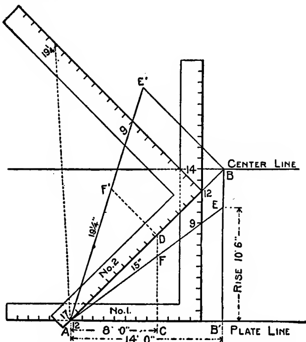
Fig. 61. Steel Square in Roof Dormer Framing.
