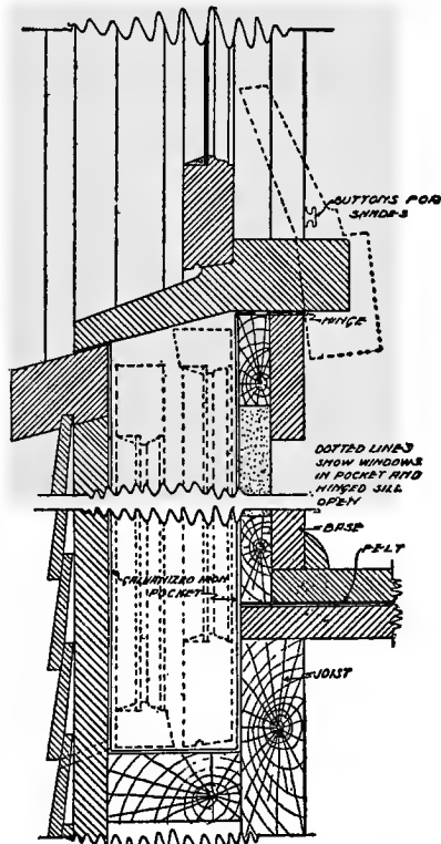
Fig. 35. Storm-Proof Box and Sill.
