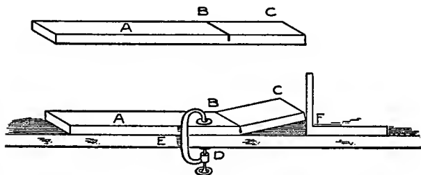
Fig. 58. To Kerf a Circular Member to Any Desired Radius.
