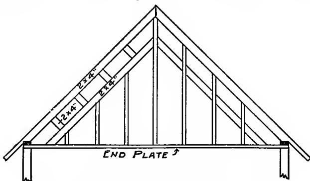
Fig. 21. Two Methods of Putting in Show Blocks.
