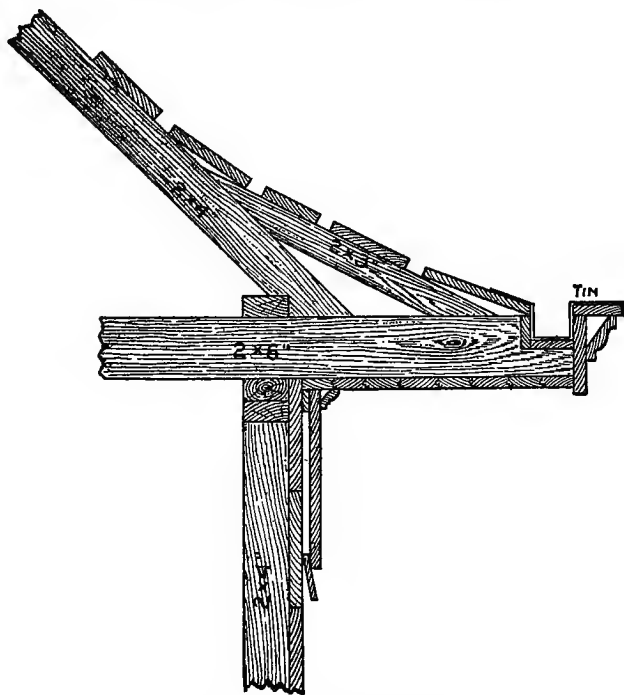
Fig. 18. Cornice Construction.
