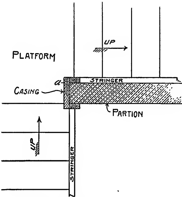
Fig. 82. Arrangement for Platform Stairs.
