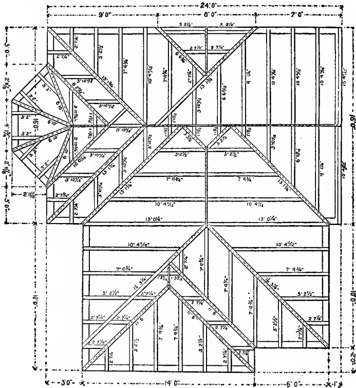
Fig. 57. Framing Plan for Hip-and-Valley Roof
