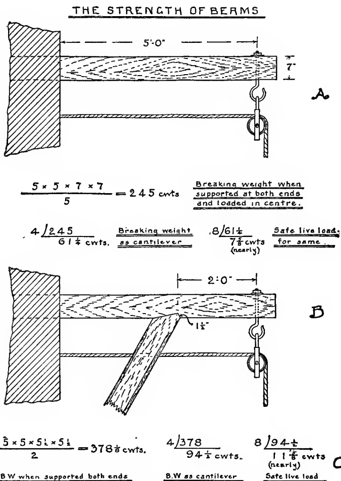
Fig. 163. Ultimate Strength of Beams Used as Braced and as Unbraced Cantilevers, Loaded at Outer End.
