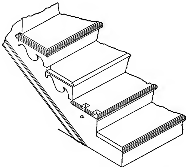
Fig. 80. Construction and Finish of Open Stairs.
