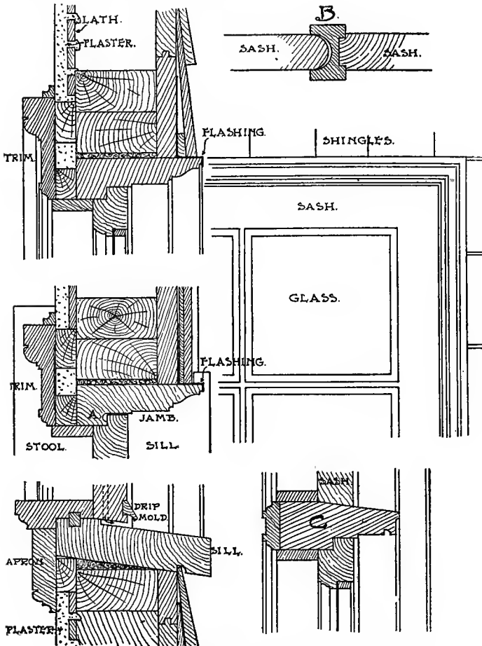
Fig. 25. Framing for Outward-Opening Casements.
