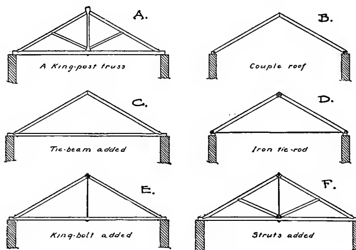
Fig. 171. Simple Roof Trusses.
